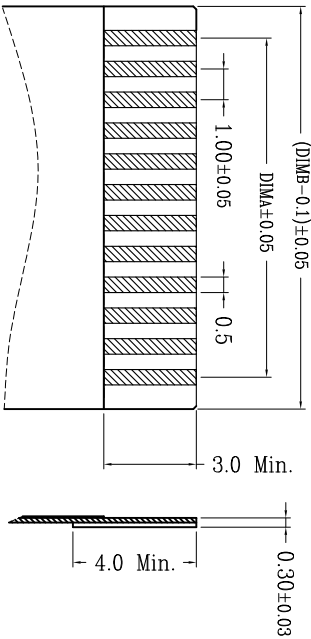
适用扁平线 (Applicable Flat Cable)
