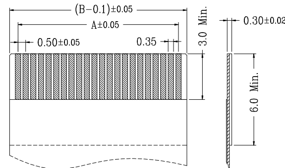
适用扁平线(Applicable Flat Cable)
